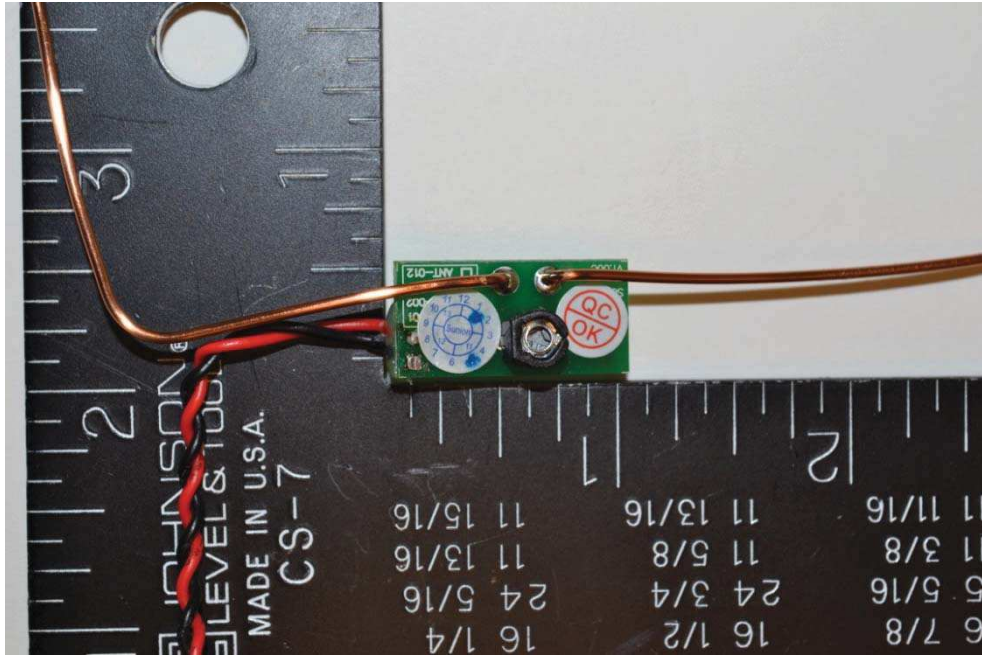
3. RFID Antenna PCB Bottom
