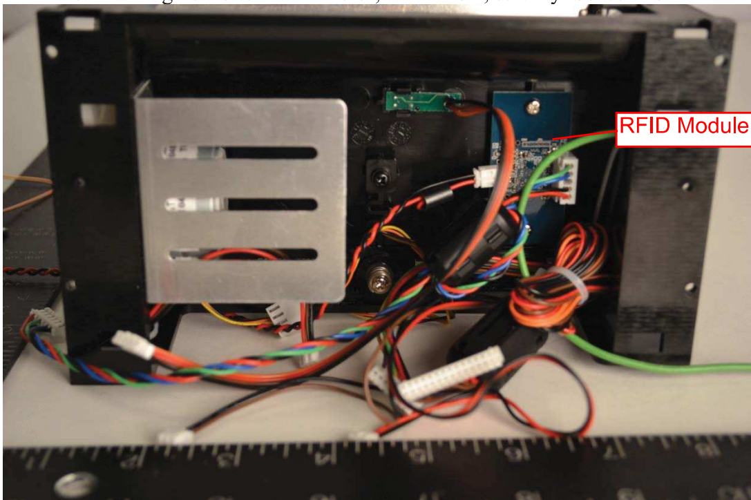
6. Engine Bottom with motor, RFID PCB, & Vinyl Sensor PCB
