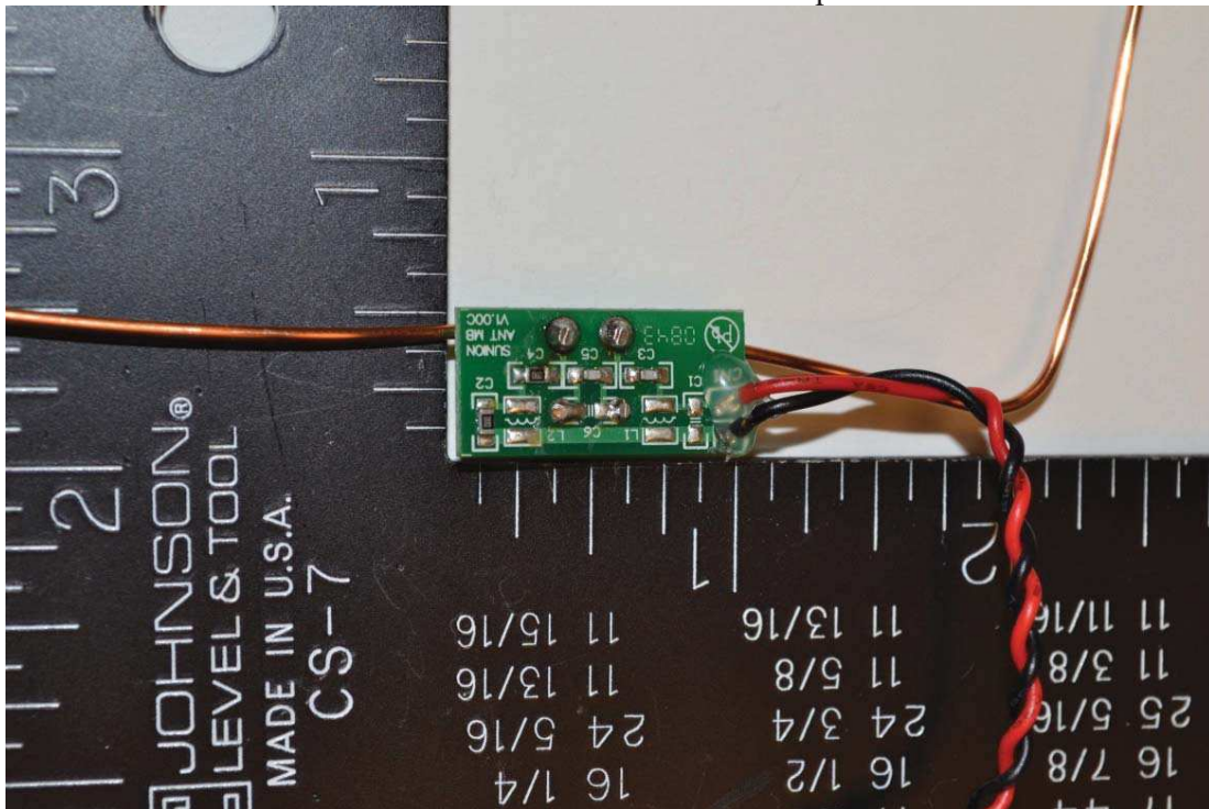
2. RFID Antenna PCB Top
