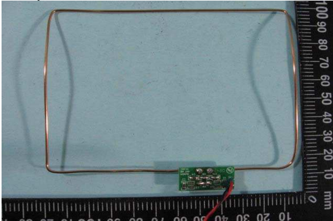
26. Component View of RFID Antenna PCB
