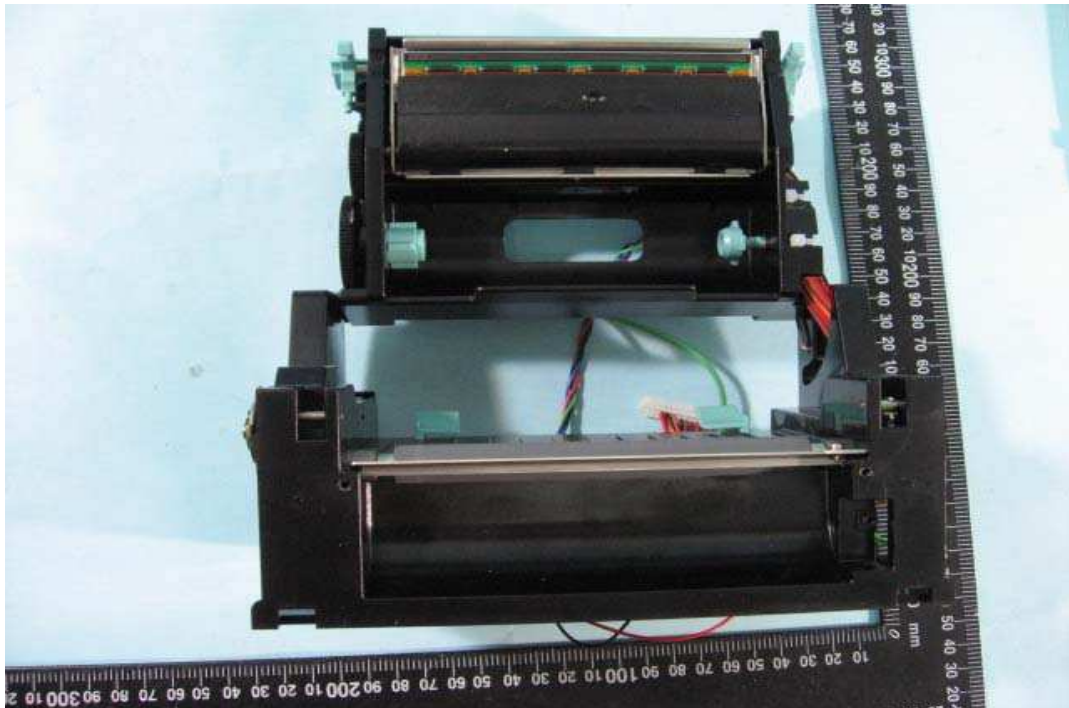
21. Internal View of EUT
