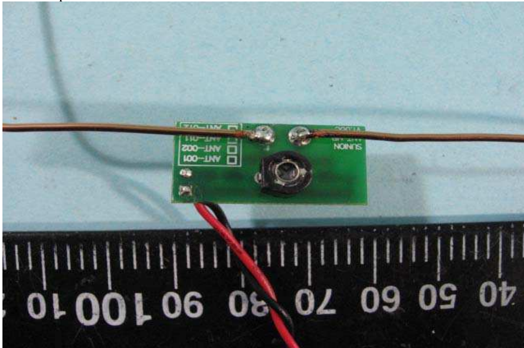
28. Component View of RFID Antenna Main PCB
