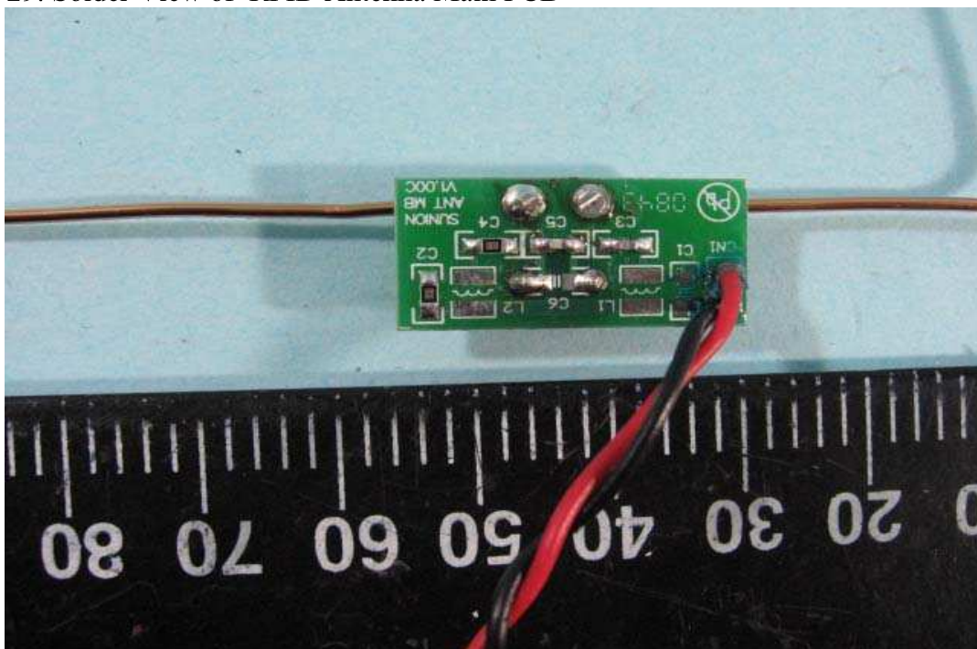
29. Solder View of RFID Antenna Main PCB
