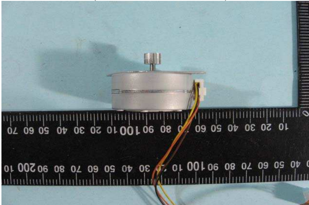
8. Total View of Motor(Motor Model: PM42L-048-XTB3)
