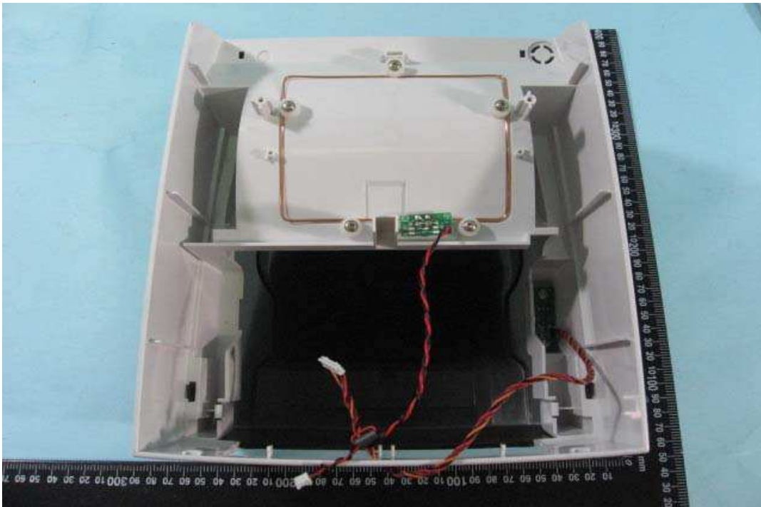
19. Internal View of EUT
