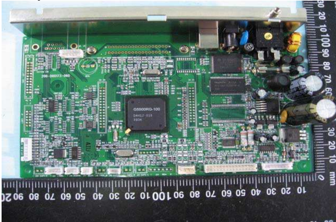
34. Component View of PCB
