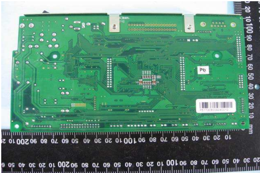
35. Solder View of PCB
