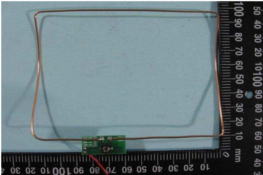
27. Solder View of RFID Antenna PCB
