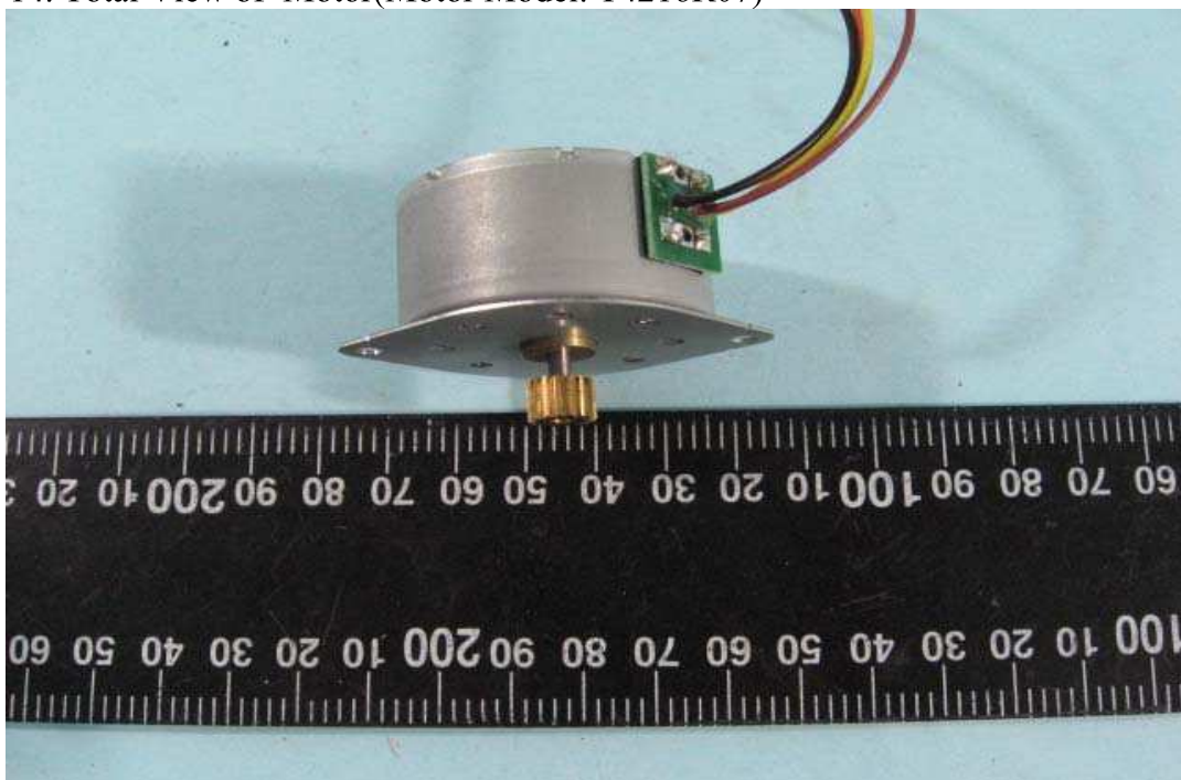
14. Total View of Motor(Motor Model: T4216R07)
