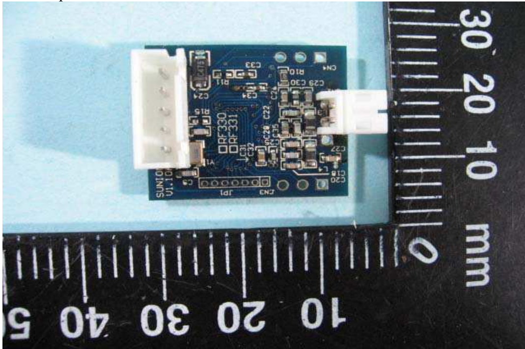
24. Component View of RFID PCB
