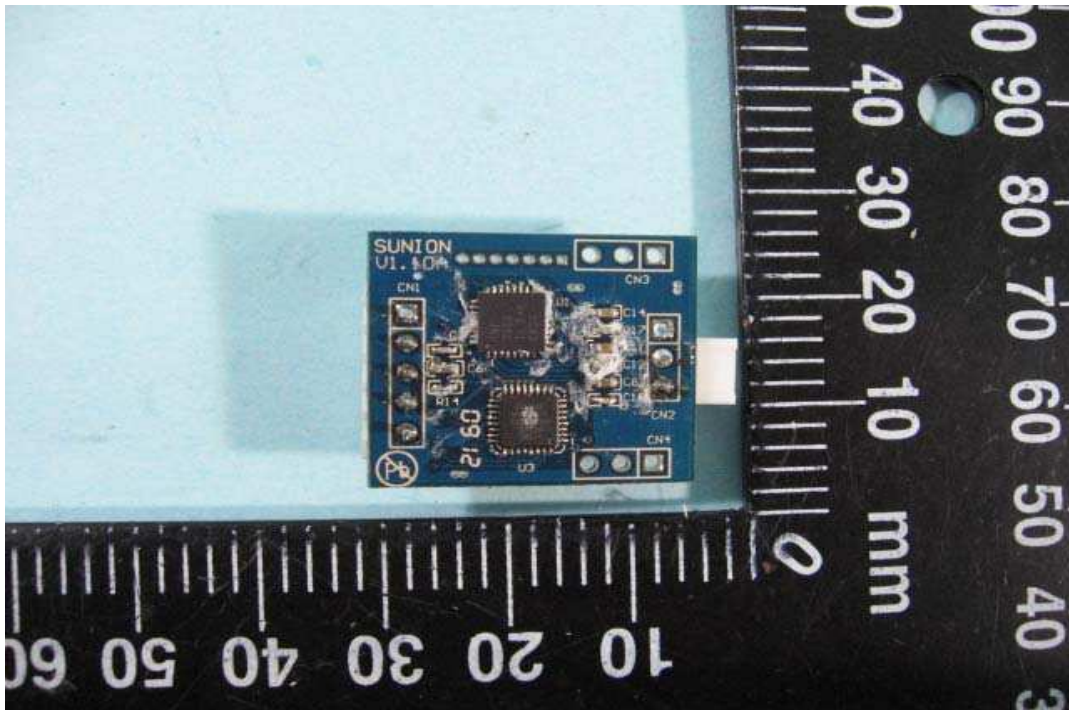
25. Solder View of RFID PCB
