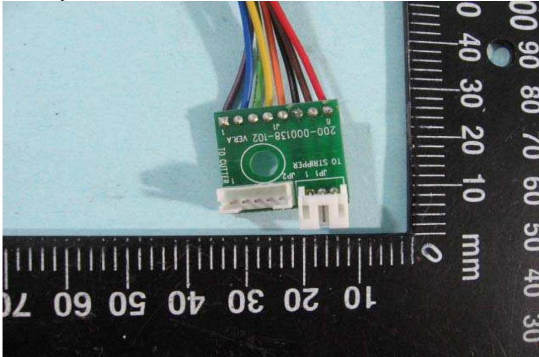
30. Component View of PCB
