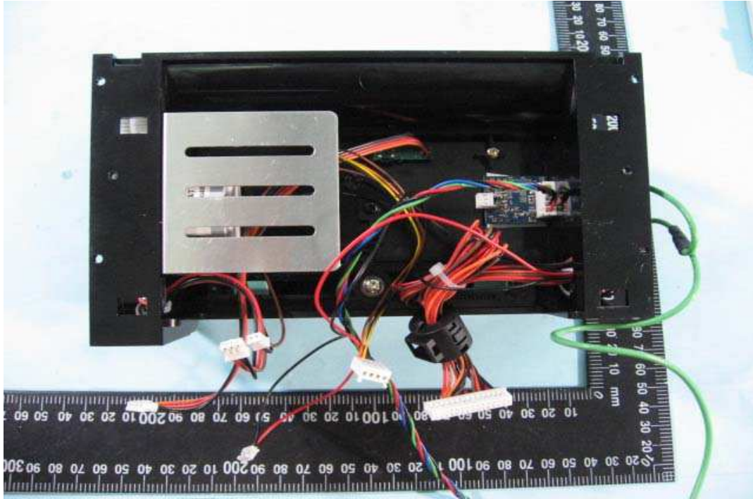
20. Internal View of EUT
