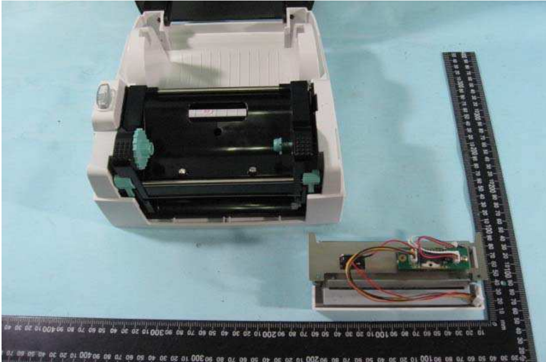
18. Internal View of EUT
